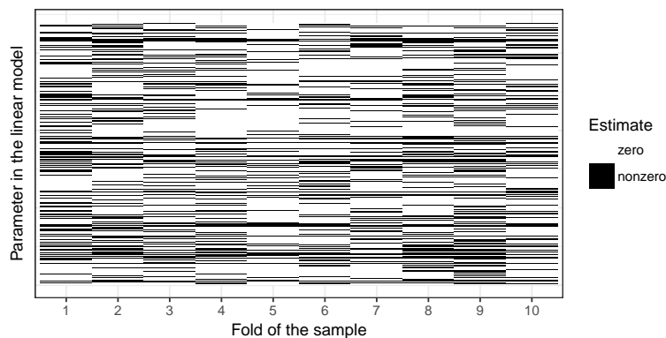
Figure 1: Features selected in across different subsets of the American Housing Survey. Figure reproduced from code from the supplementary materials of Sendhil Mullainathan and Jann Spiess, "Machine Learning: An Applied Econometric Approach," Journal of Economic Perspectives 31, no. 2 (2017): 87-106, doi: 10.1257/jep.31.2.87 .
